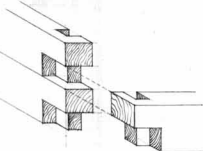
INBUCCAREA GRINZILOR 1/10
